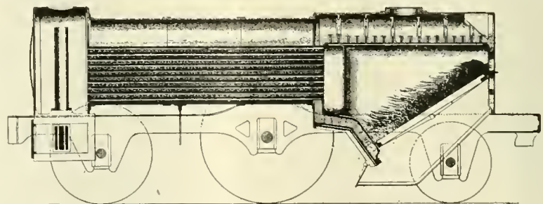
CUDWORTH'S COAL BURNING BOILER. FIG. 54.
